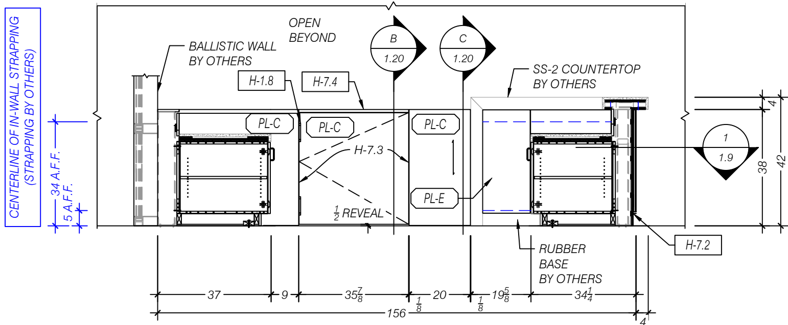
1 ELEVATION NORTH - RECEPTION SCALE 1:32 (3/8"=1'-0") ARCH REF: 3/AE580
