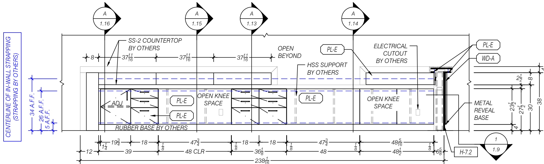
2 ELEVATION EAST - RECEPTION SCALE 1:32 (3/8"=1'-0") ARCH REF: 4/AE580
